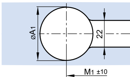
8-12NMT View A-A: Recess in the frame plate
