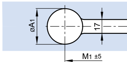
4-6NMT View A-A: Recess in the frame plate
